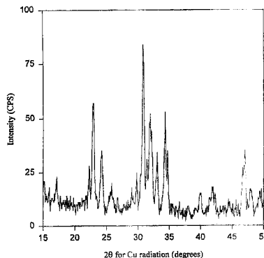
X-Ray Diffraction Spectrum (θ-2θ) of powder prepared from the Ca-P colloid with silicon as the introduced additive. Approximate phase ratio: 33 ± 5% HA and 67 ± 5% Si-TCF.
