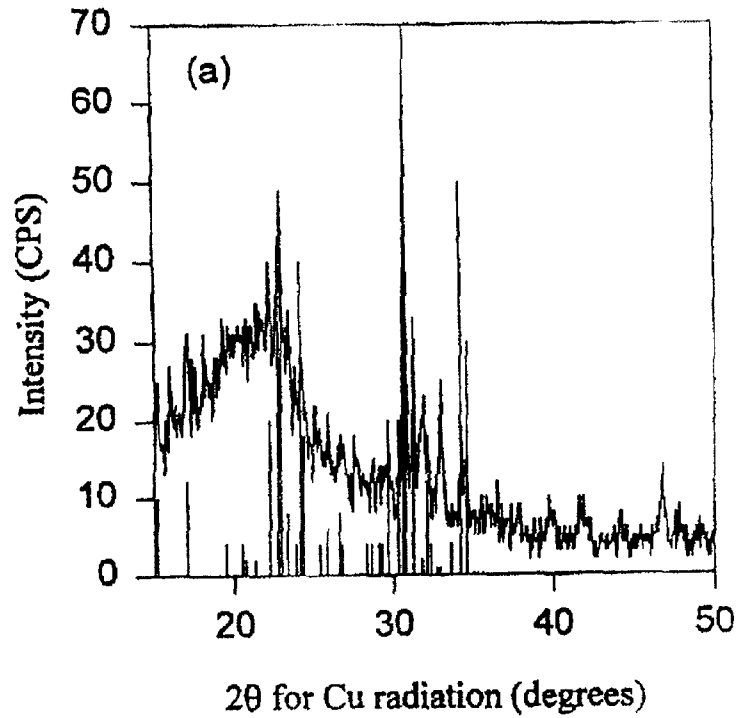
Figure 2: Glancing Angle X-Ray Diffraction Spectra of a thin film of the Ca-P colloid sintered on quartz at 1000°C. (a) Overlay of JCPDS#9-348 ( \alpha -TCP). (b) Overlay of JCPDS#9-432 (HA).
